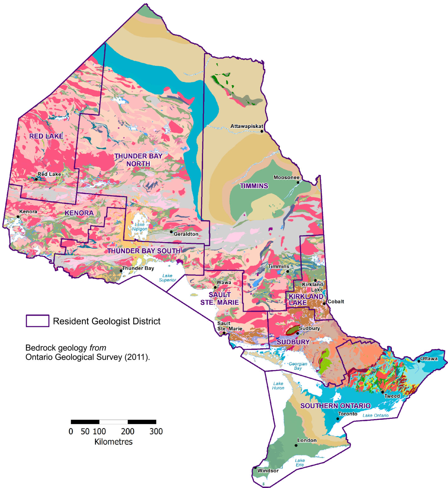
Ontario Geological Survey 2011. 1:250 000 scale bedrock geology of Ontario; Ontario Geological Survey, Miscellaneous Release—Data 126 – Revision 1.
