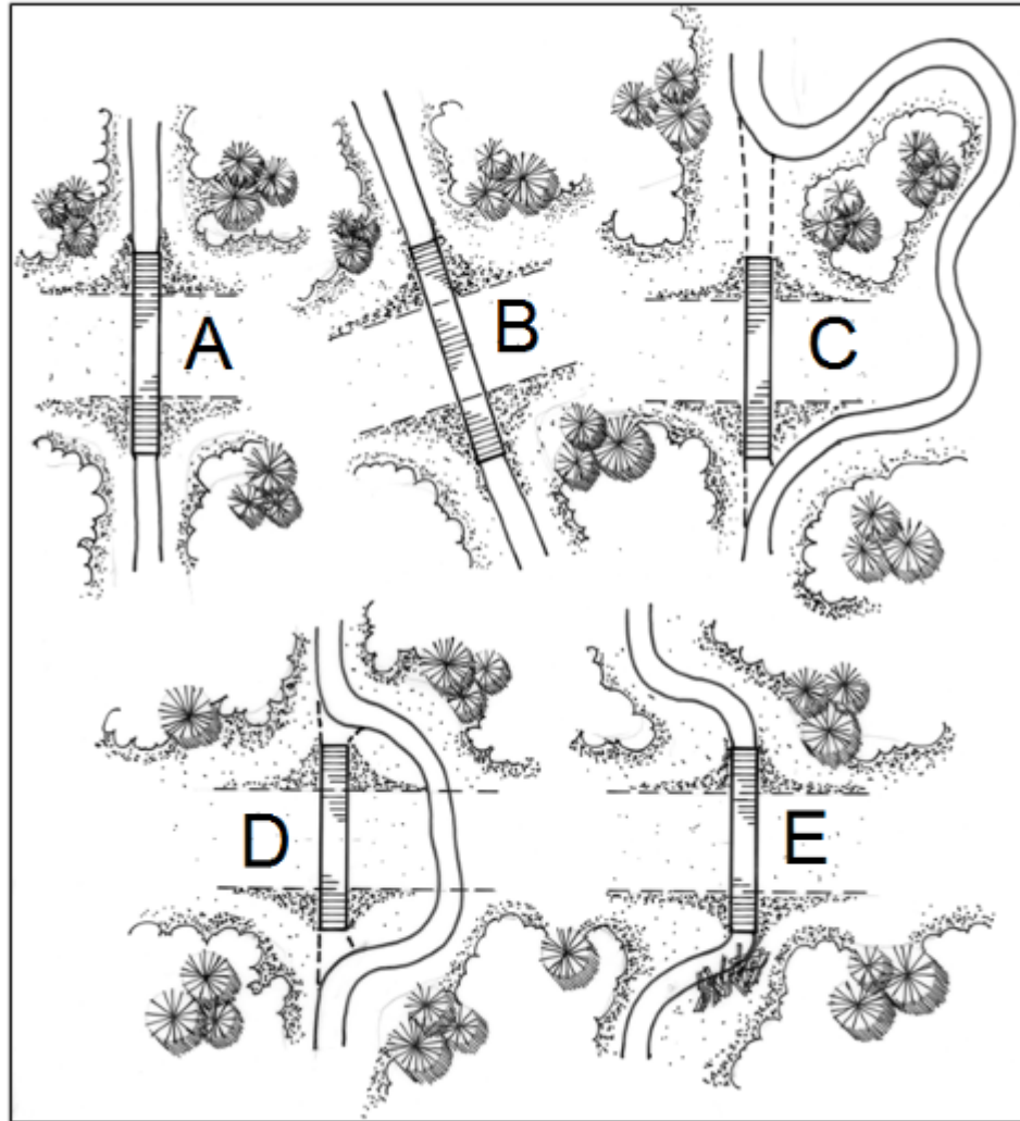
Figure 5.1b. Fitting a culvert to the creek alignment to minimize change in stream morphology. Examples A, B, and E are preferred. Examples C and D change stream morphology and will likely require DFO approval (Illustration by Kestevan Design).
