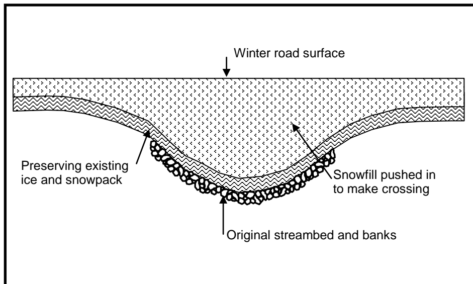
Figure 5.1d. An example of a temporary winter snowfill crossing.
