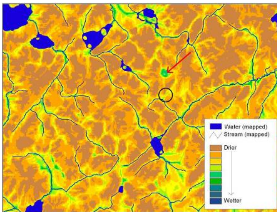
Figure 5.2d. Example of a topographic index map used to predict relative wetness. The red arrow indicates a predicted wet area that would not have been obvious from visual inspection of topographic maps. The black circle indicates the predicted location of a concentrated drainage path. Knowing these locations in advance allows for more robust operational planning (season of harvest, equipment selection, road and skid trail layout, etc.).
