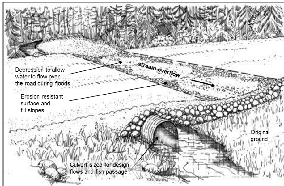
Figure 5.1f. A depression beside the culvert allows water to spill over the road in the event of a flood or culvert blockage (Illustration by Kestevan Design).
