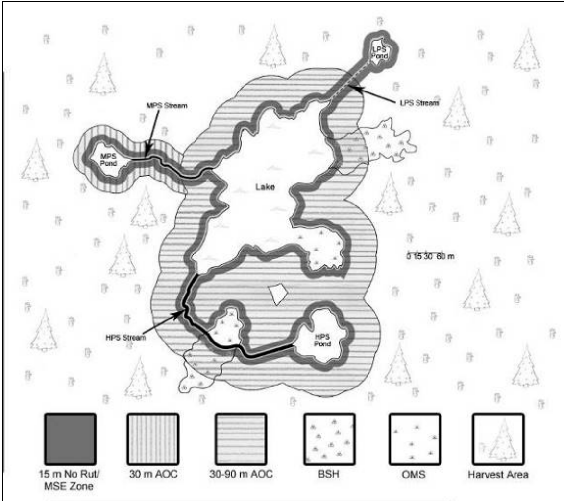
Figure 4.1a. Layout of areas of concern (AOC) and 15 m no rut or significant mineral soil exposure (MSE) zones around lakes, ponds, and streams. Ponds/streams with high (HPS), moderate (MPS), or low (LPS) potential sensitivity to forest management operations are identified (see Sections 4.1.1 and 4.1.2). (Illustration by Mandy Saille).
